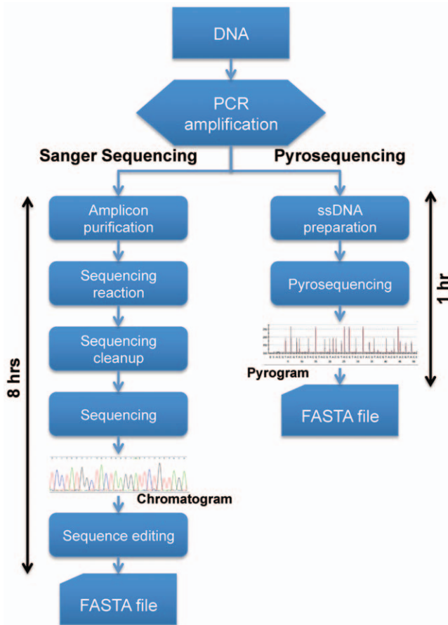
Figure 2. Schematic representation of pyrosequencing vs. Sanger sequencing workflows. doi:10.1371/journal.pone.0021252.g002
