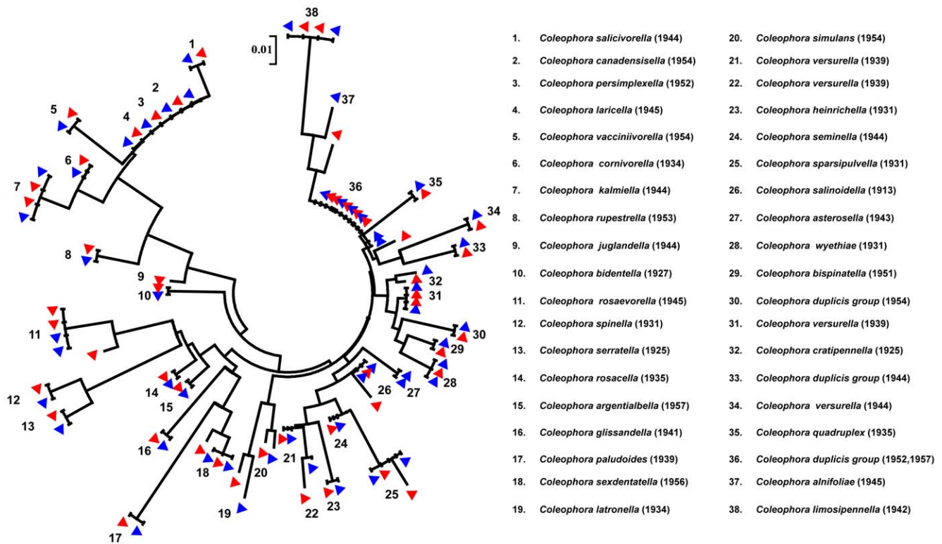
Figure 1. Neighbor-joining (NJ) trees based on Kimura-2-Parameter (K2P) distances for cytochrome c oxidase I (COI) mini-barcodes of old museum Lepidoptera specimens. The red markers indicate the position of generated pyrosequences in comparison to the reference library, with blue markers, from BOLD or Genbank. Collection dates are shown in parentheses. doi:10.1371/journal.pone.0021252.g001
