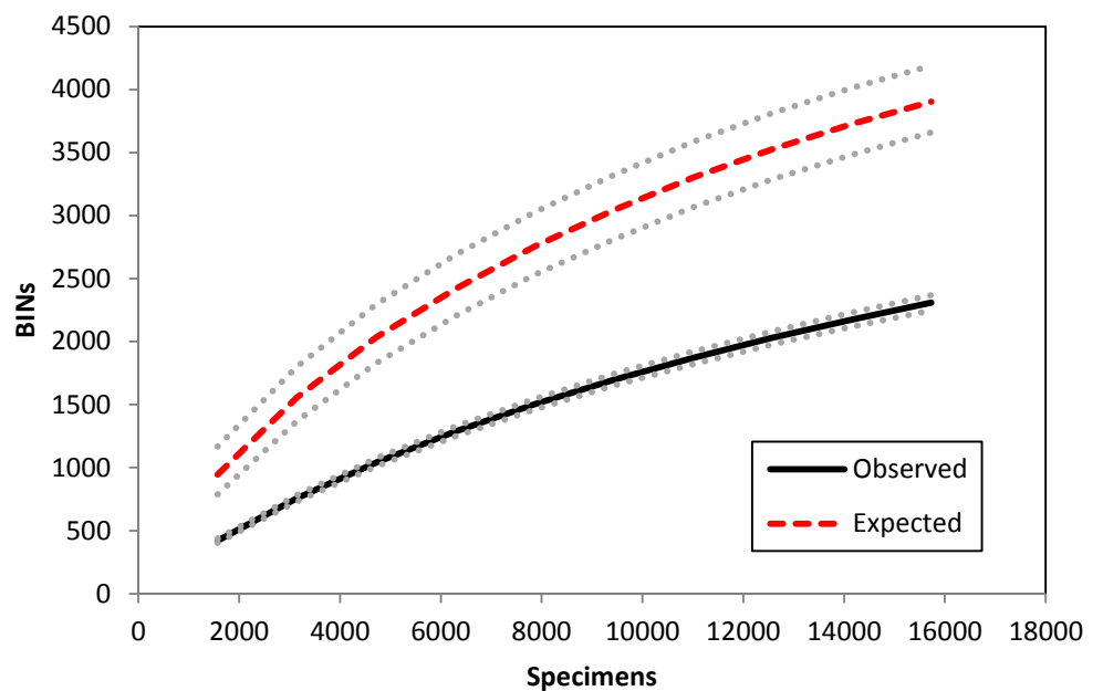
Figure 16. BIN accumulation curve for all specimens collected by the Malaise traps at Gros Morne National Park in 2013.
