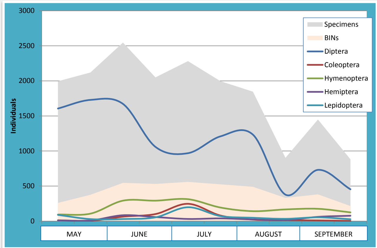
Figure 18. Seasonal variation of the major insect orders as well as specimen and BIN counts collected at Gros Morne National Park in 2013.
