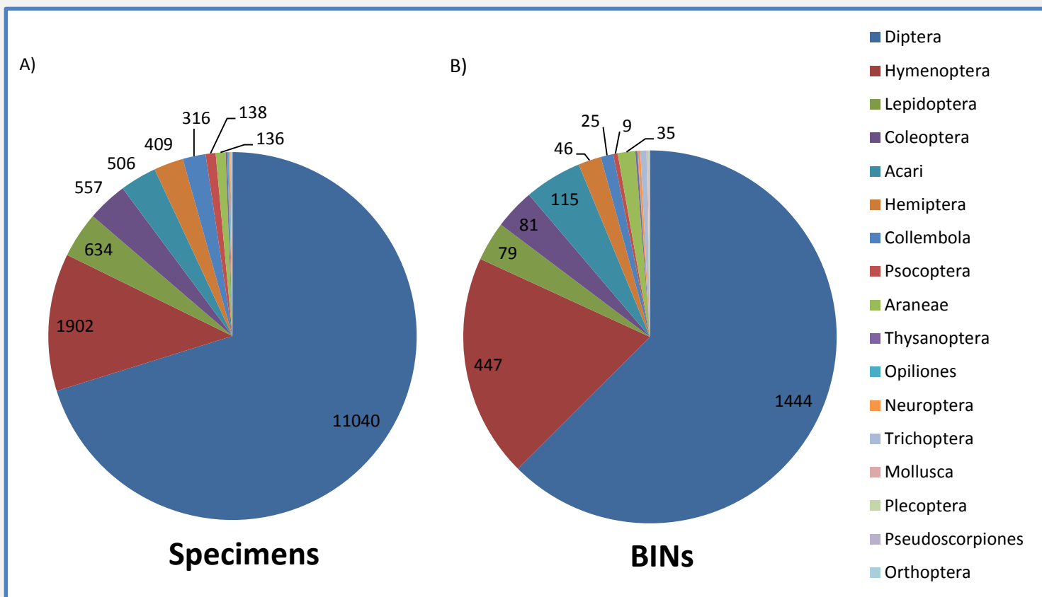
Figure 15. Taxonomic breakdown of (A) N total specimens and (B) N total BINs collected by Malaise traps at Gros Morne National Park in 2013.
