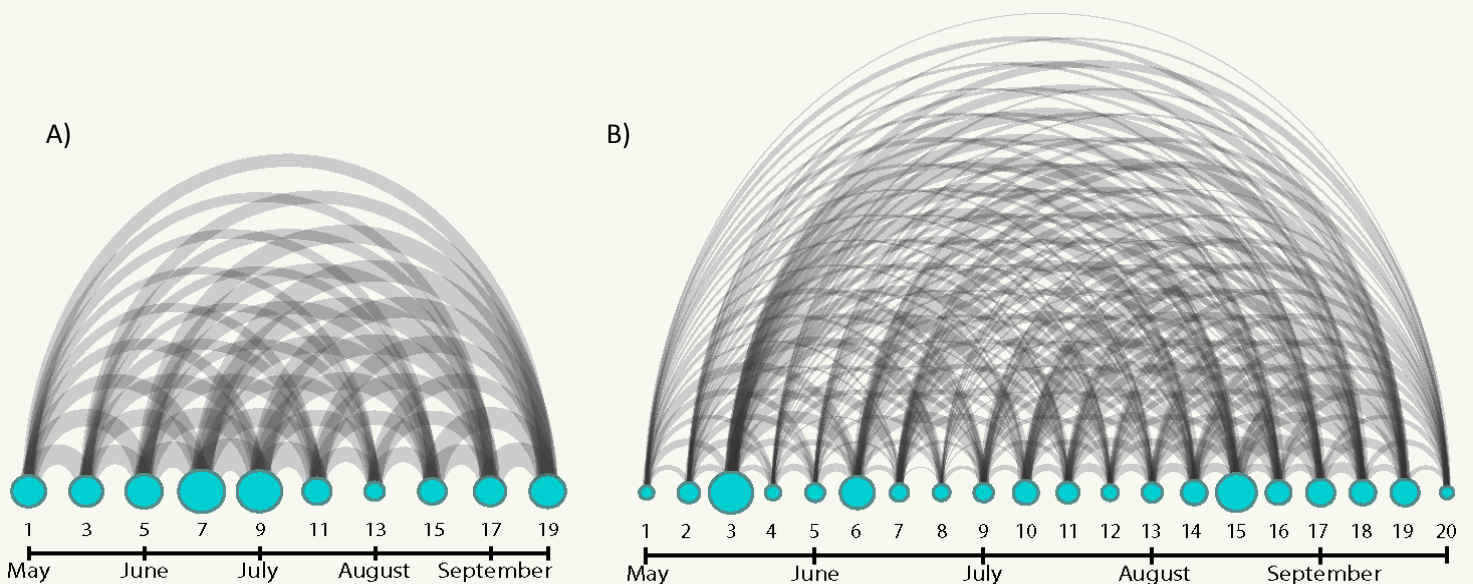
Figure 11. Species overlap between A) 10 bi-weekly samples collected in Point Pelee National Park in 2012, and B) 20 weekly samples collected in Rouge National Park in 2013. Size of nodes indicate the number of BINs in each sample, and the width of the arcs reflect the number of species shared between each sample.
