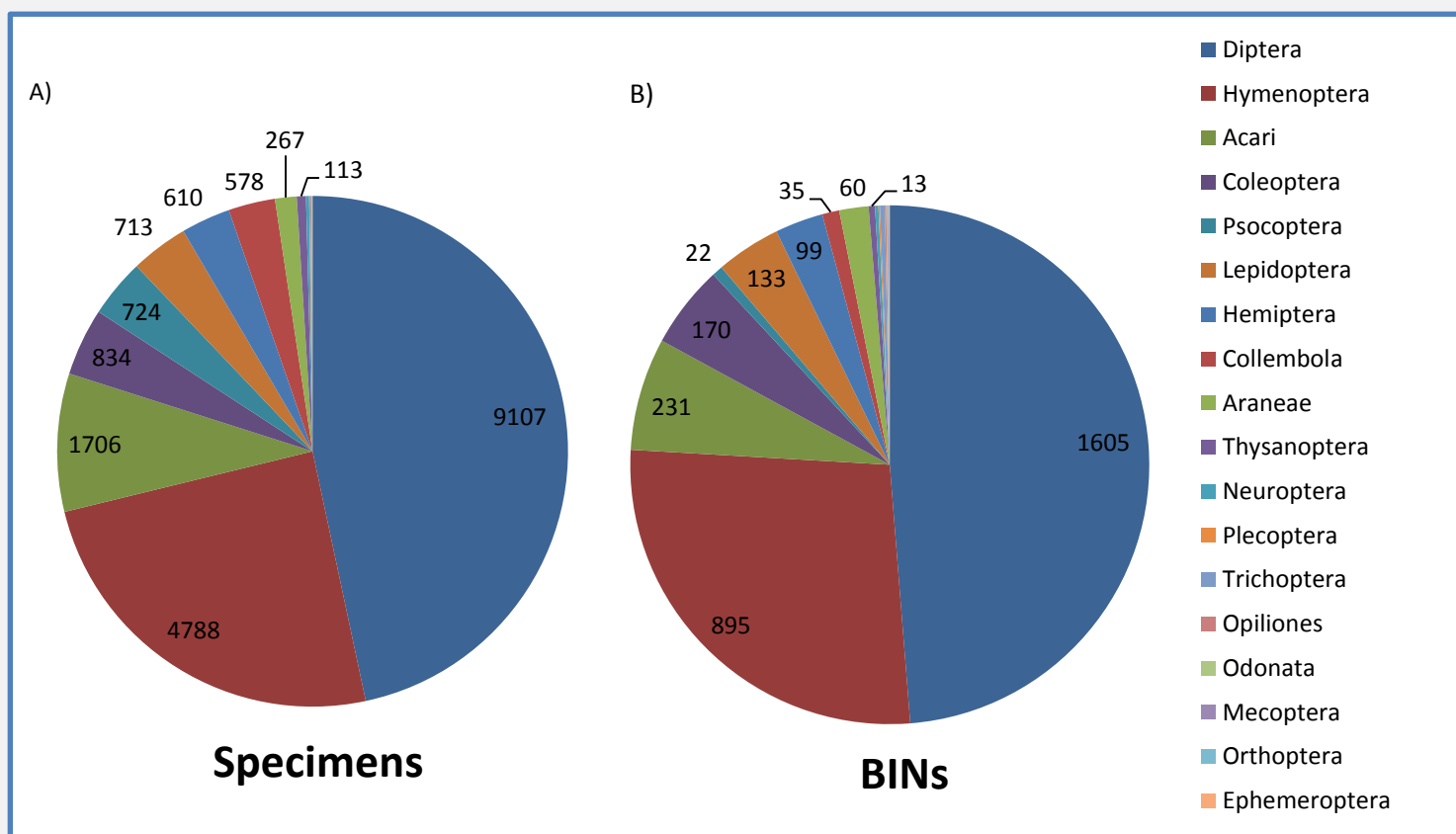
Figure 15. Taxonomic breakdown of (A) N total specimens and (B) N total BINs collected by Malaise traps at La Mauricie National Park in 2013.
