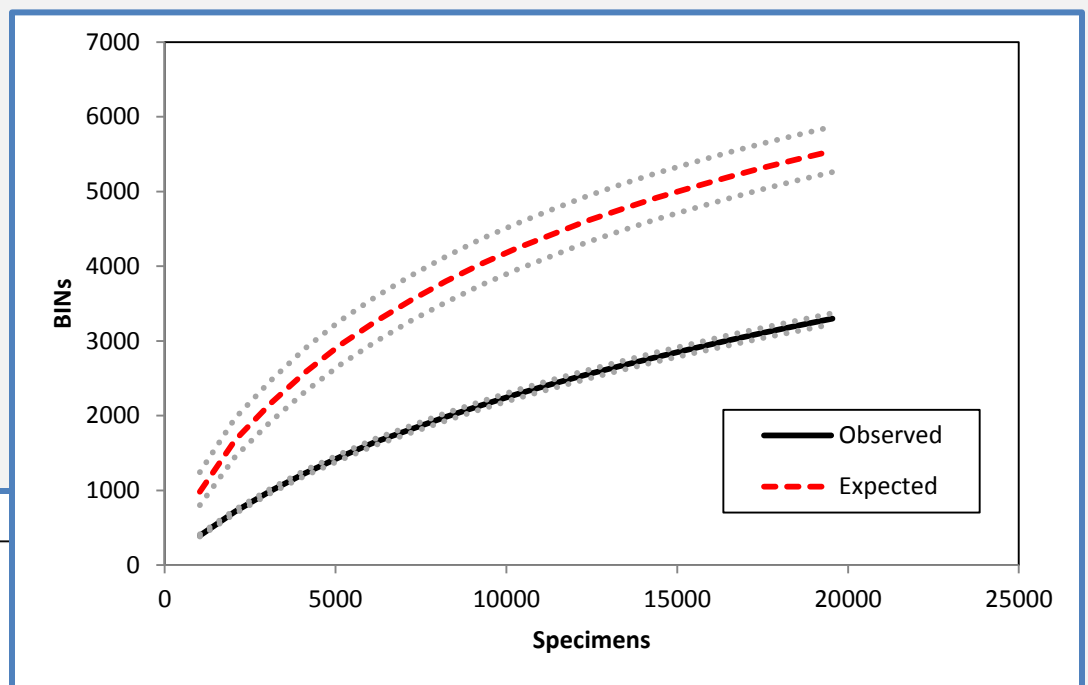
Figure 16. BIN accumulation curve for all specimens collected by the Malaise traps at La Mauricie National Park in 2013.
