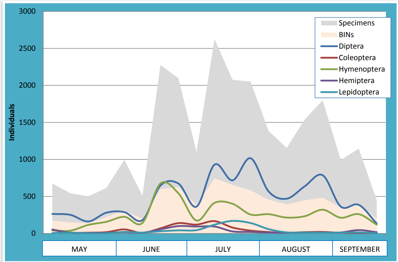
Figure 18. Seasonal variation of the major insect orders as well as specimen and BIN counts collected at La Mauricie National Park in 2013.
