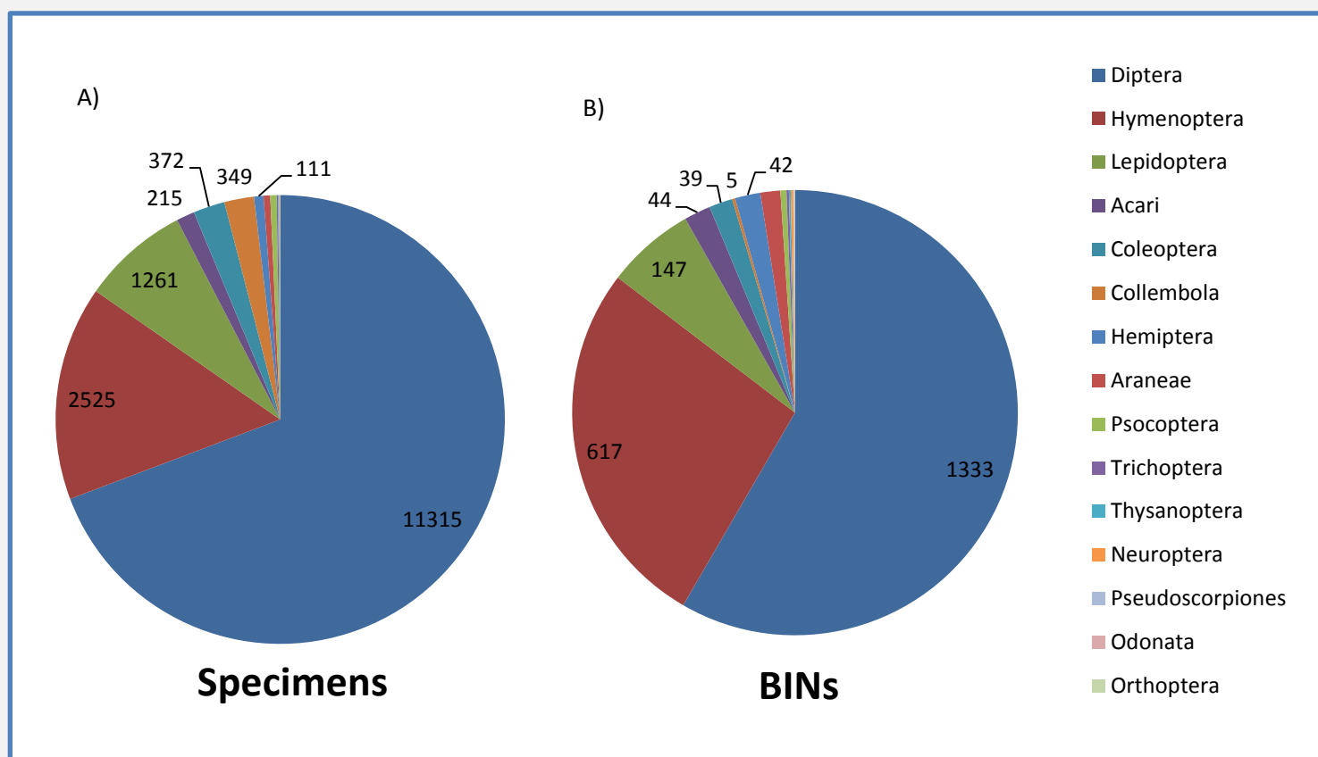
Figure 15. Taxonomic breakdown of (A) N total specimens and (B) N total BINs collected by Malaise traps at Mingan Archipelago National Park in 2013.
