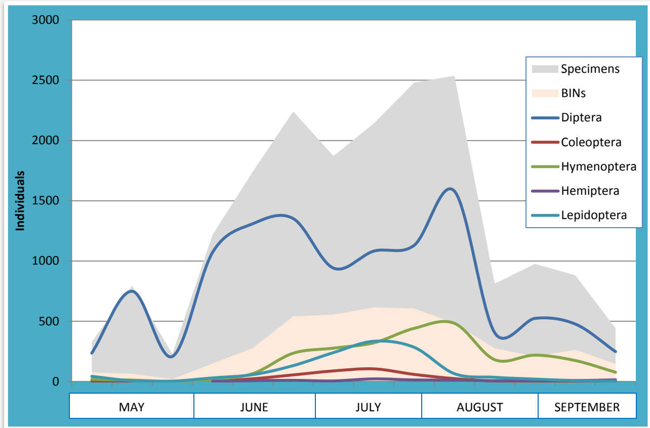
Figure 18. Seasonal variation of the major insect orders as well as specimen and BIN counts collected at Mingan Archipelago National Park in 2013.
