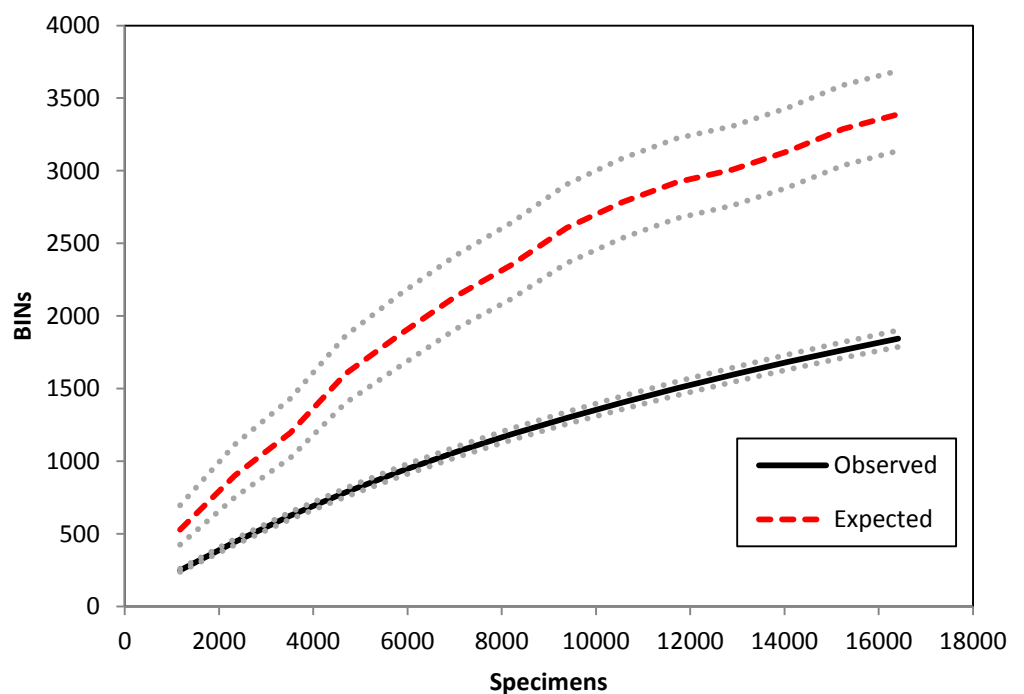
Figure 16. BIN accumulation curve for all specimens collected by the Malaise traps at Mingan Archipelago National Park in 2013.
