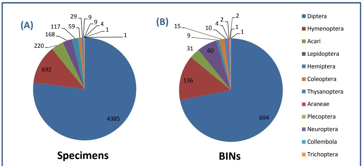
Figure 16. Taxonomic breakdown of (A) 5694 total specimens and (B) 965 total BINs collected by Malaise traps at Ivavik National Park in 2014.
