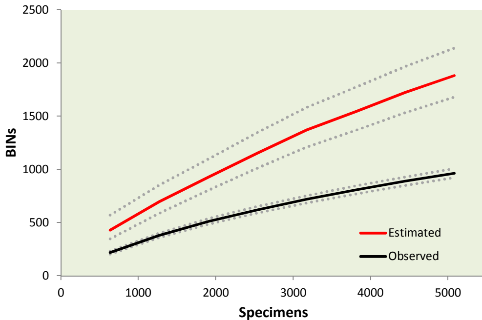
Figure 17. BIN accumulation curve for all specimens collected by the Malaise traps at Ivavik National Park in 2014.
