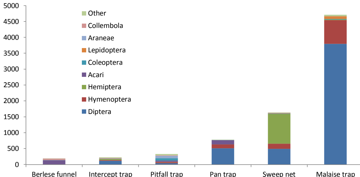
Figure 19. Total number of specimens sorted out so far from the standardized sampling collections at Kluane National Park in 2014. Colours indicate the taxonomic breakdown captured using different collecting methods.
