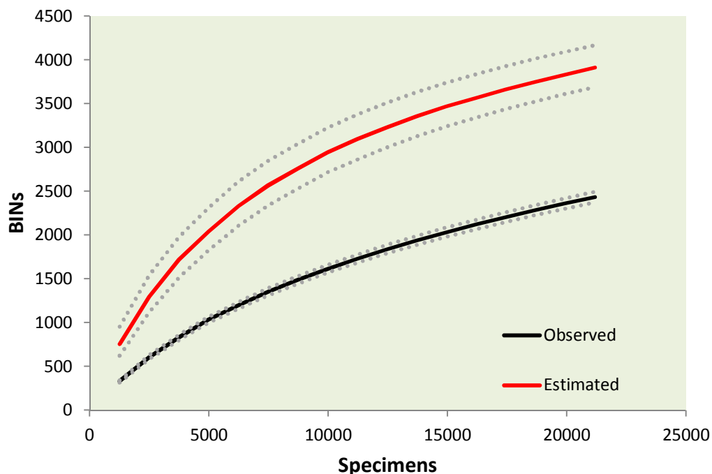
Figure 17. BIN accumulation curve for all specimens collected by the Malaise traps at Kluane National Park in 2014.
