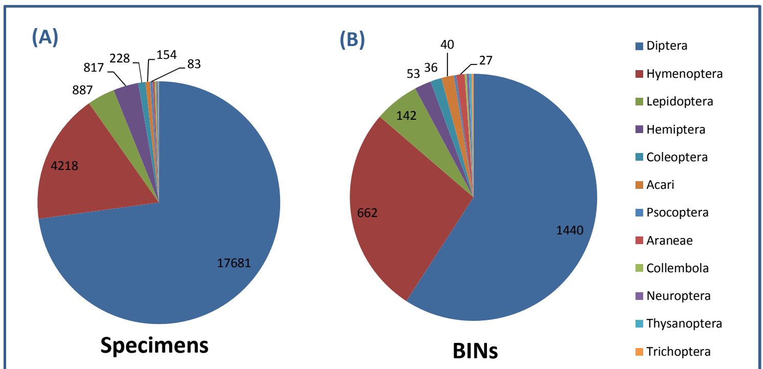
Figure 16. Taxonomic breakdown of (A) 24,263 total specimens and (B) 2435 total BINs collected by Malaise traps at Kluane National Park in 2014.
