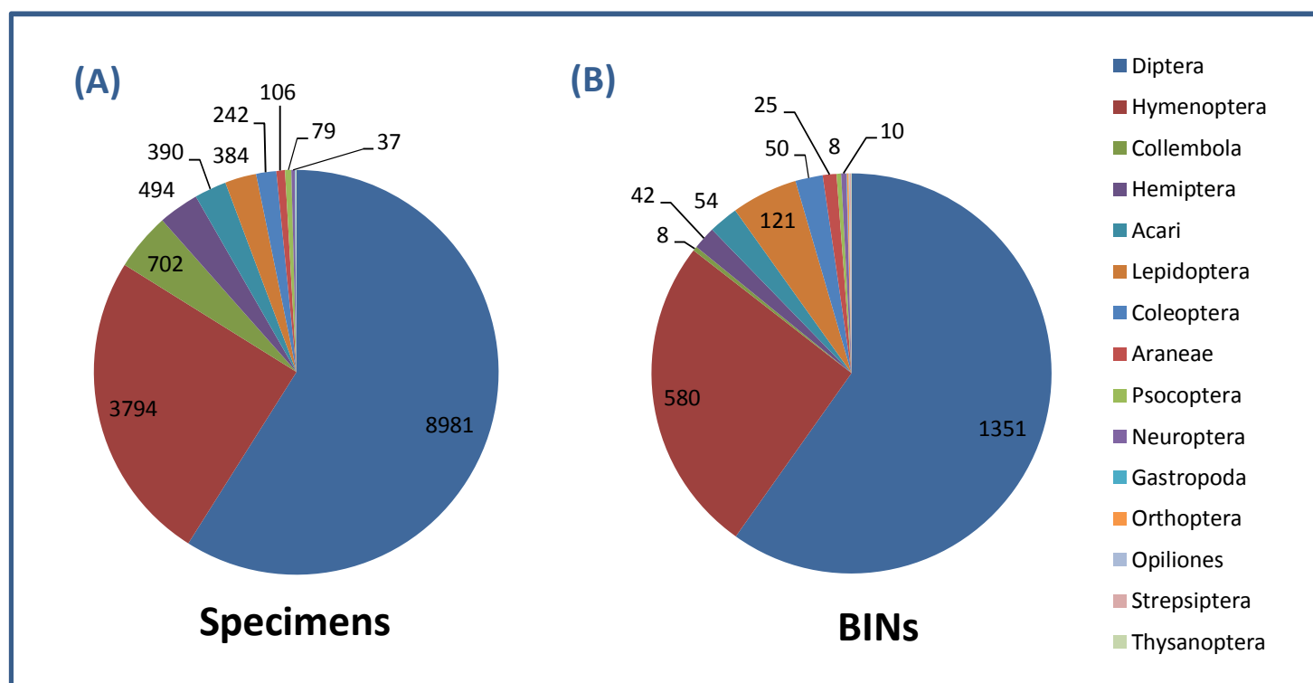
Figure 16. Taxonomic breakdown of (A) 15,228 total specimens and (B) 2258 total BINs collected by Malaise traps at Kootenay National Park in 2014.
