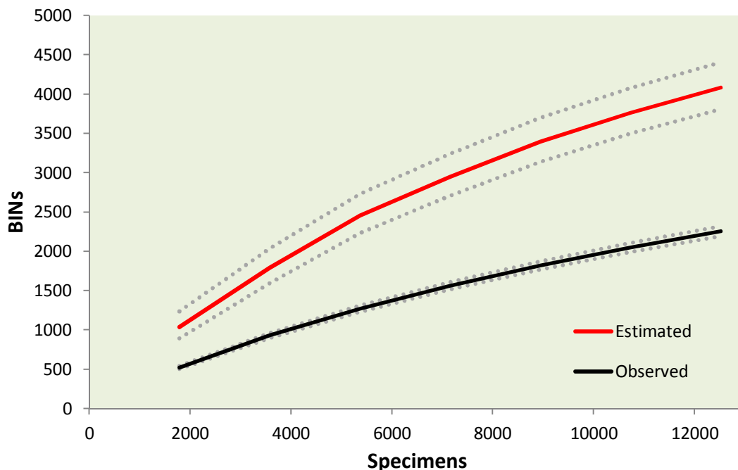
Figure 17. BIN accumulation curve for all specimens collected by the Malaise traps at Kootenay National Park in 2014.
