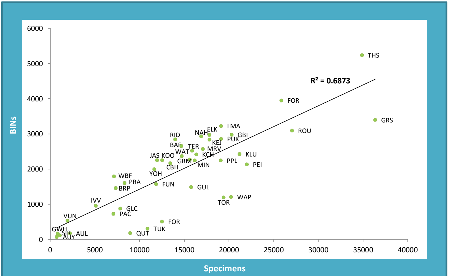
Figure 8. Regression analysis examining the relationship between the number of barcoded specimens and number of BINs (BINs = 0.1187(Specimens) + 243.18).
