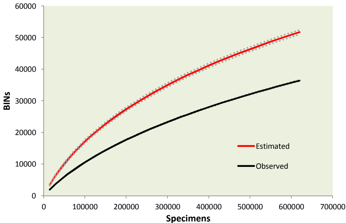
Figure 4. BIN accumulation curve for the 746 Malaise trap samples collected in 43 Canadian National Parks during 2012-2014.
