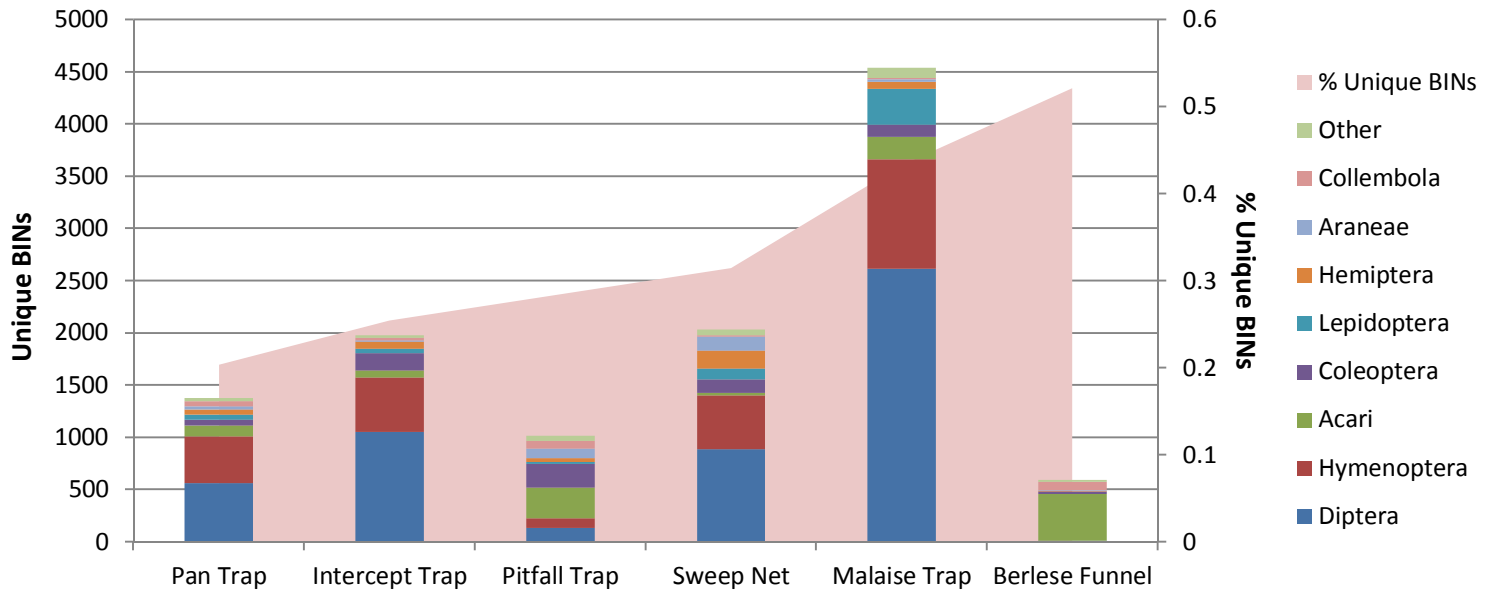
Figure 14. Total number of BINs unique to each collecting method and their taxonomic breakdown (bars) and the percentage of unique BINs collected with each method (Unique BINs/Total BINs).
