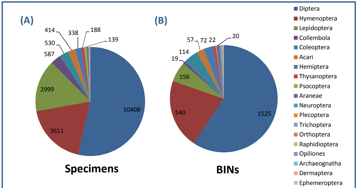
Figure 16. Taxonomic breakdown of (A) 19,422 total specimens and (B) 2569 total BINs collected by Malaise traps at Mount Revelstoke National Park in 2012 and 2014.
