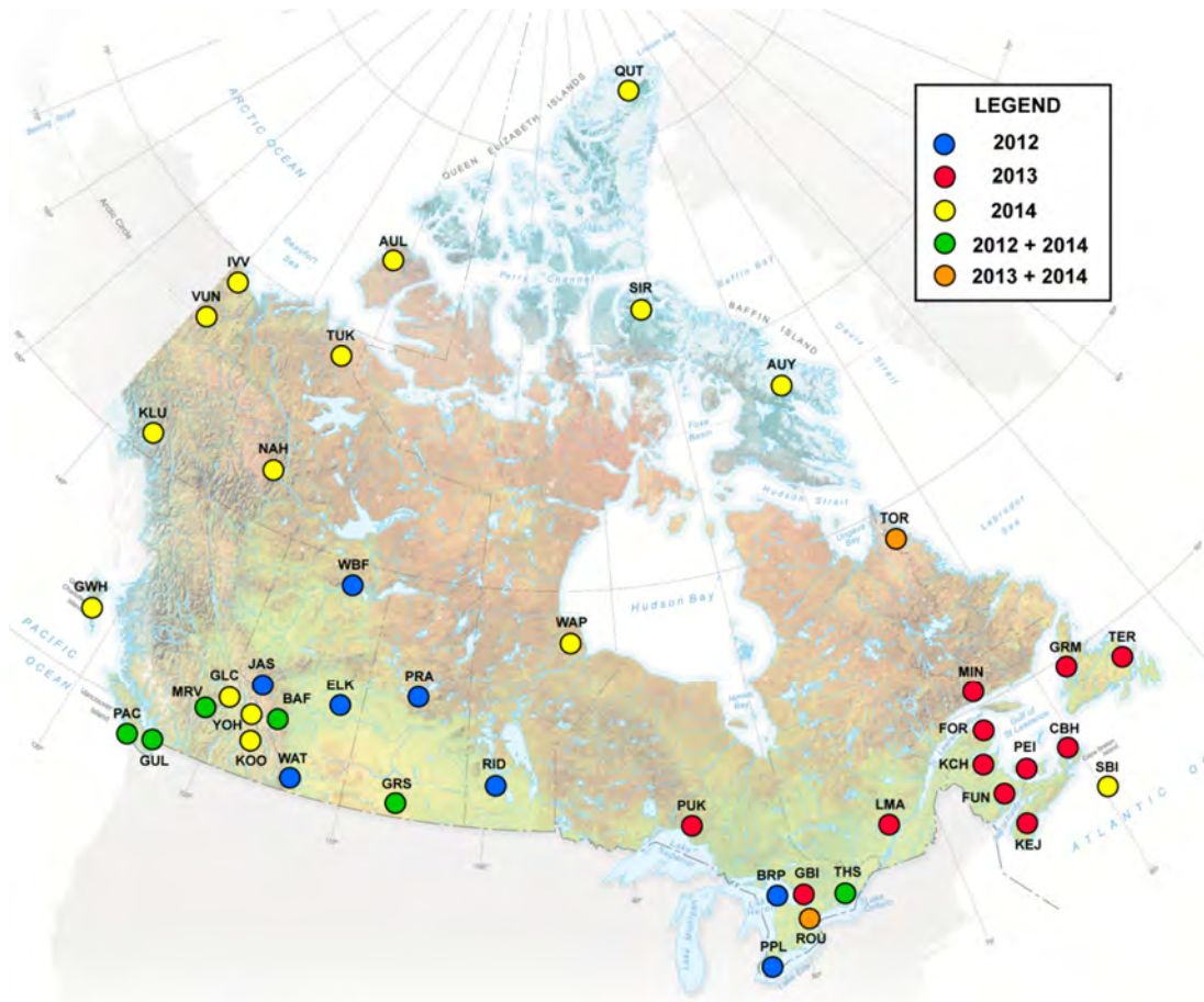
Figure 1. CNP Malaise Program sampling sites from 2012-2014.
