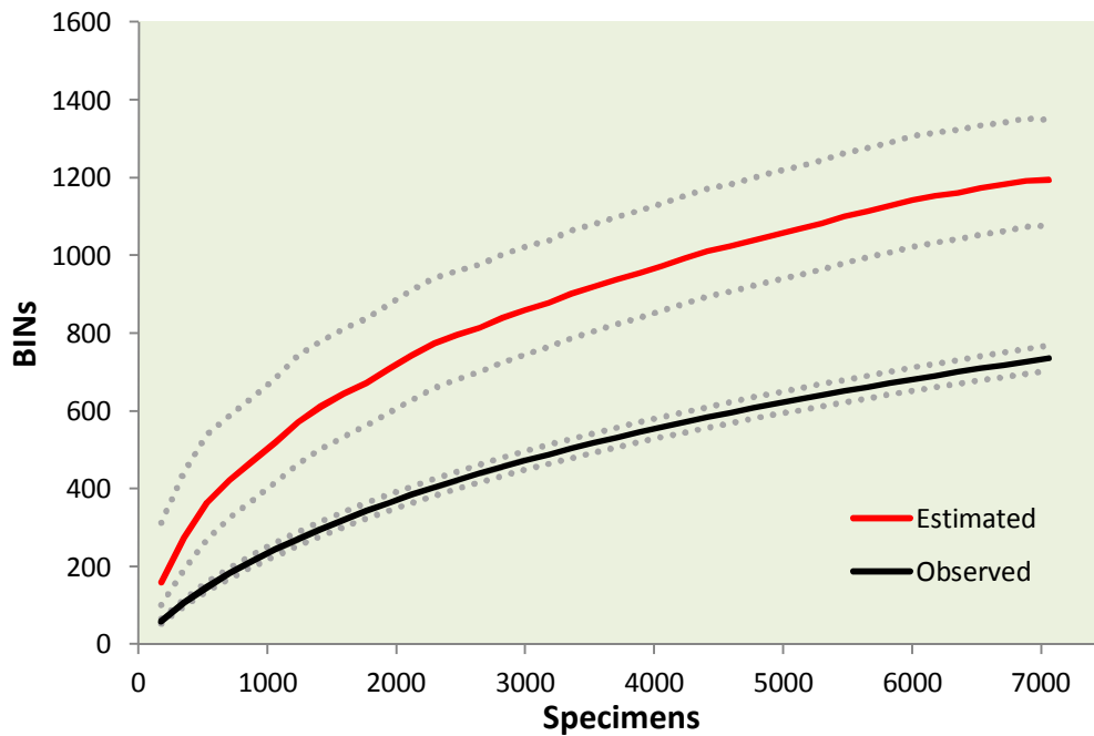
Figure 17. BIN accumulation curve for all specimens collected by the Malaise traps at Pacific Rim National Park in 2012 and 2014.
