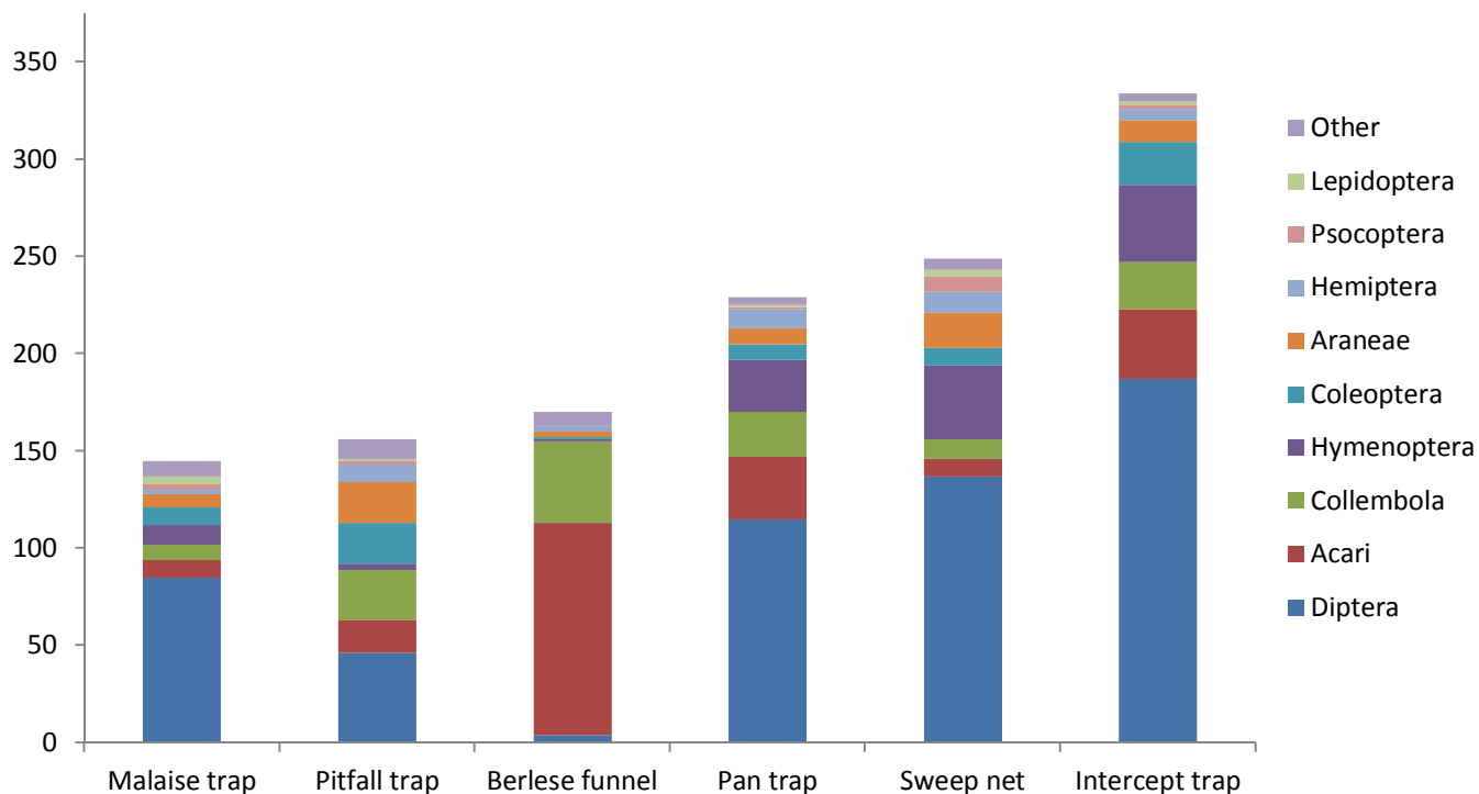
Figure 19. Total number of BINs captured (with colours indicating taxonomic breakdown) using different collecting methods through the standardized sampling program at Pacific Rim National Park in 2014.
