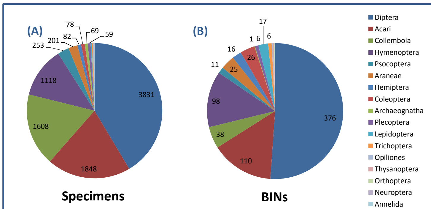
Figure 16. Taxonomic breakdown of (A) 9237 total specimens and (B) 736 total BINs collected by Malaise traps at Pacific Rim National Park in 2012 and 2014.
