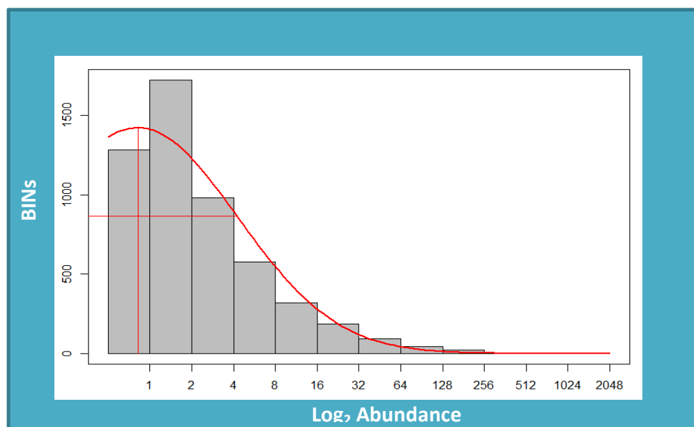
Figure 18. Lognormal species abundance curve, showing the total BINs within each \log_2 abundance frequency interval (Preston, 1962).
