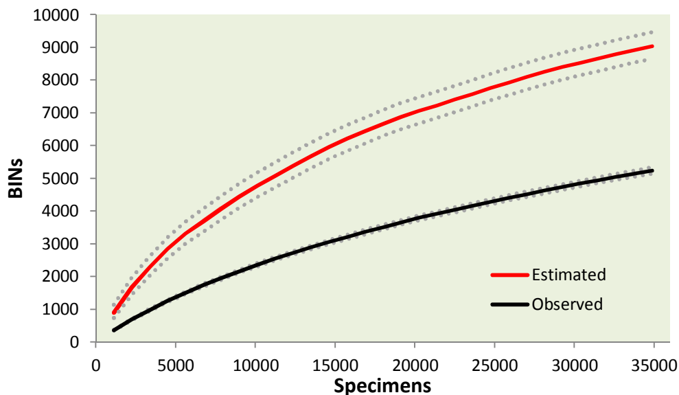
Figure 17. BIN accumulation curve for all specimens collected by the Malaise traps at Thousand Islands National Park in 2012 and 2014.
