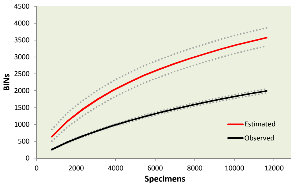
Figure 17. BIN accumulation curve for all specimens collected by the Malaise traps at Yoho National Park in 2014.
